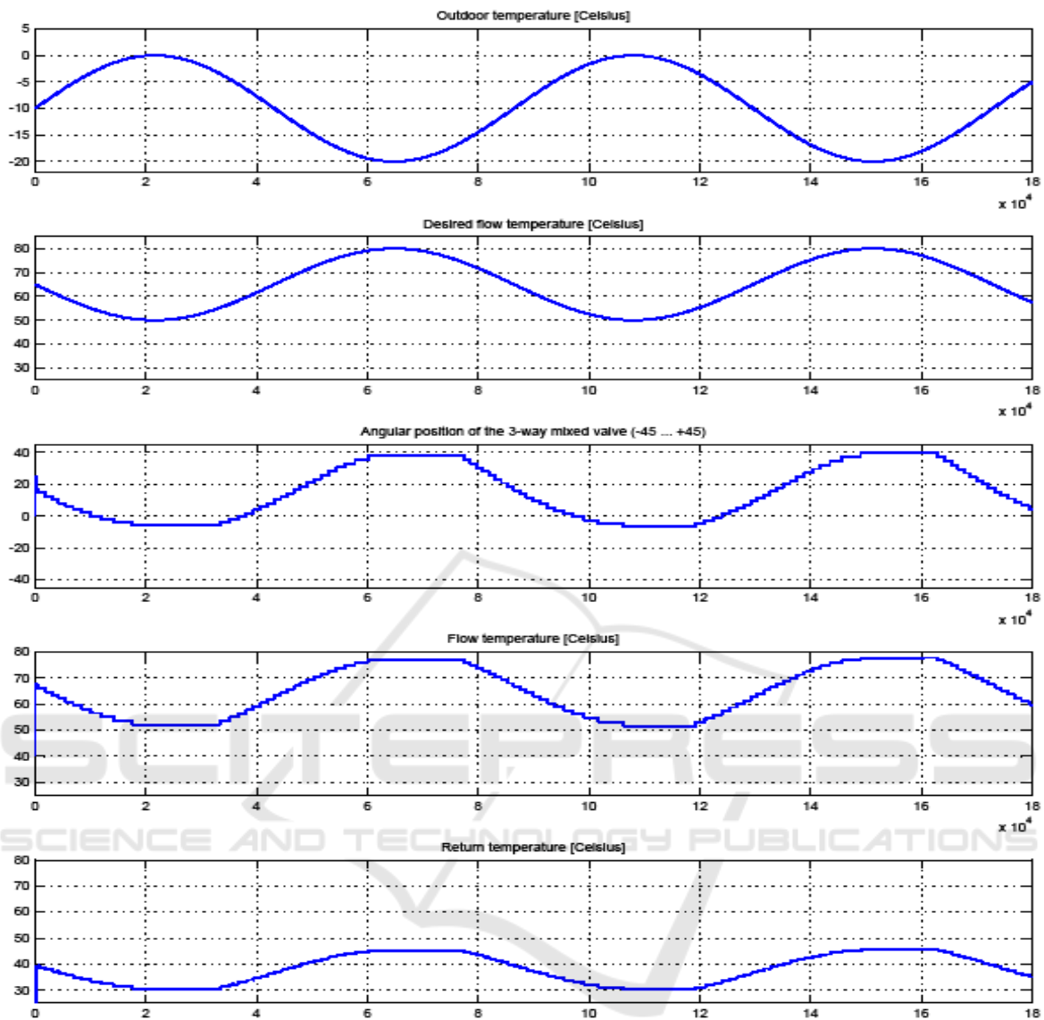
Figure 7: Results obtained by simulation of the automatic control system.
