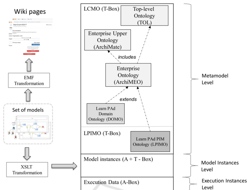
Figure 2: Ontology Levels and Transformations.
