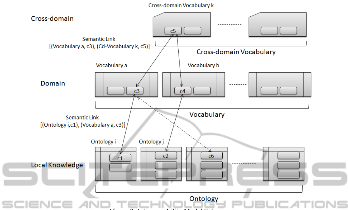
Figure 2: Interoperability Model Schema.
