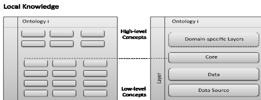
Figure 3: Local Knowledge Model.
