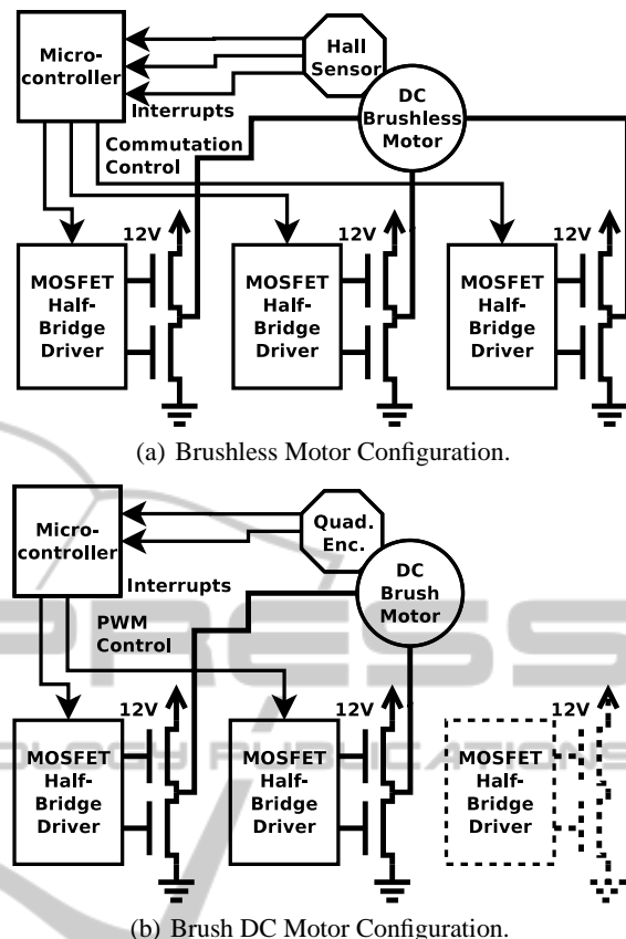
Figure 5: DC motor controller basic configurations.
