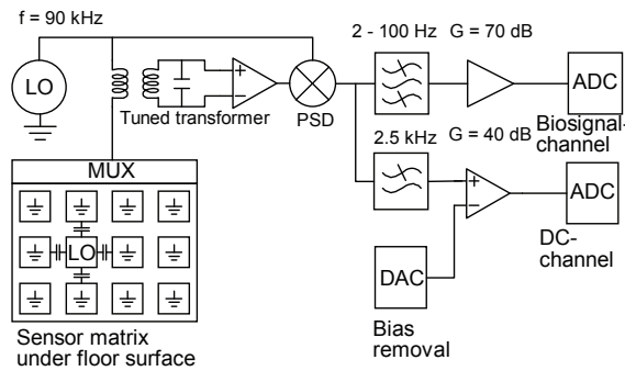
Figure 1: Block diagram of the measurement system. The local oscillator (LO) signal is fed to one sensor element at a time using an array of multiplexers.
