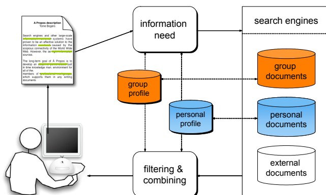
Figure 3: The À Propos architecture.
