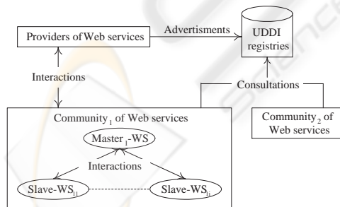
Figure 1: Architecture of Web services communities.
