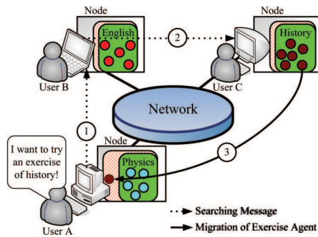
Figure 1: Proposed e-Learning system.
